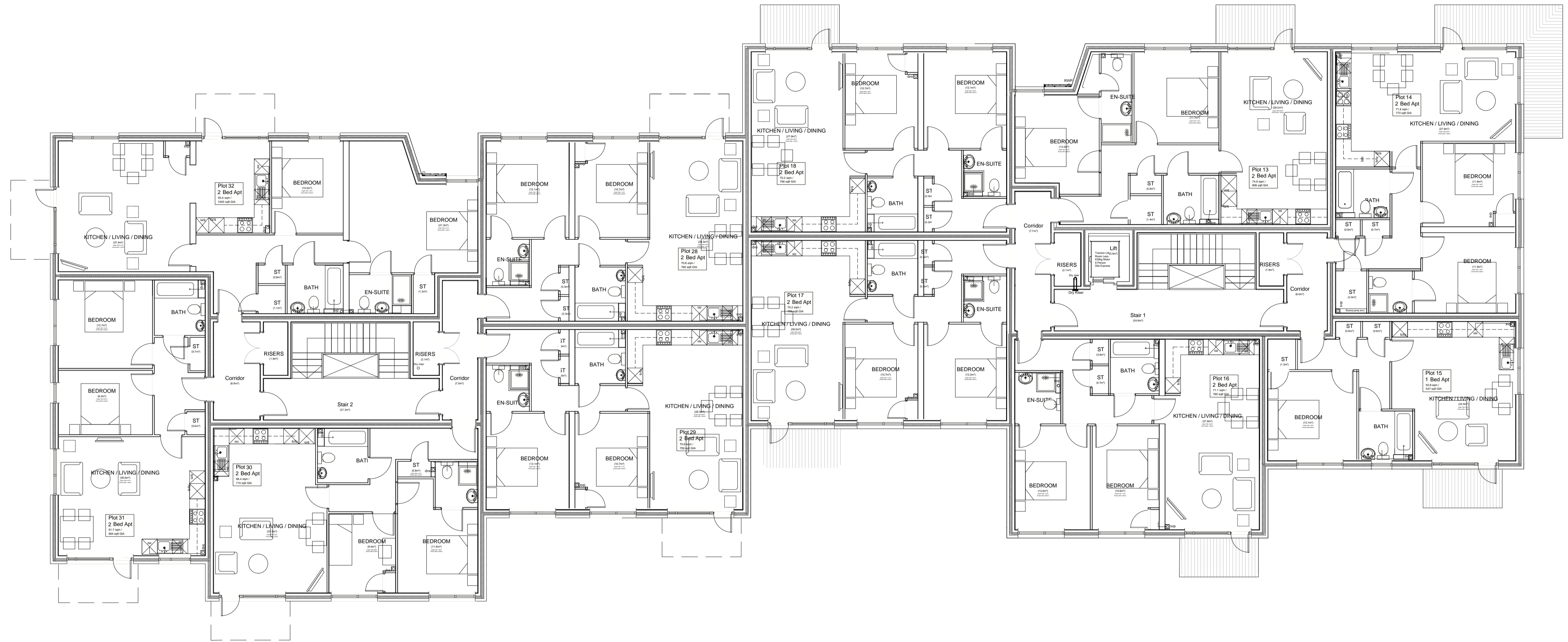
First Floor GIA (912.1m 2 )
