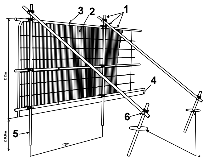
5 Figure 2: Default specification for protective barrier BS5837:2012
