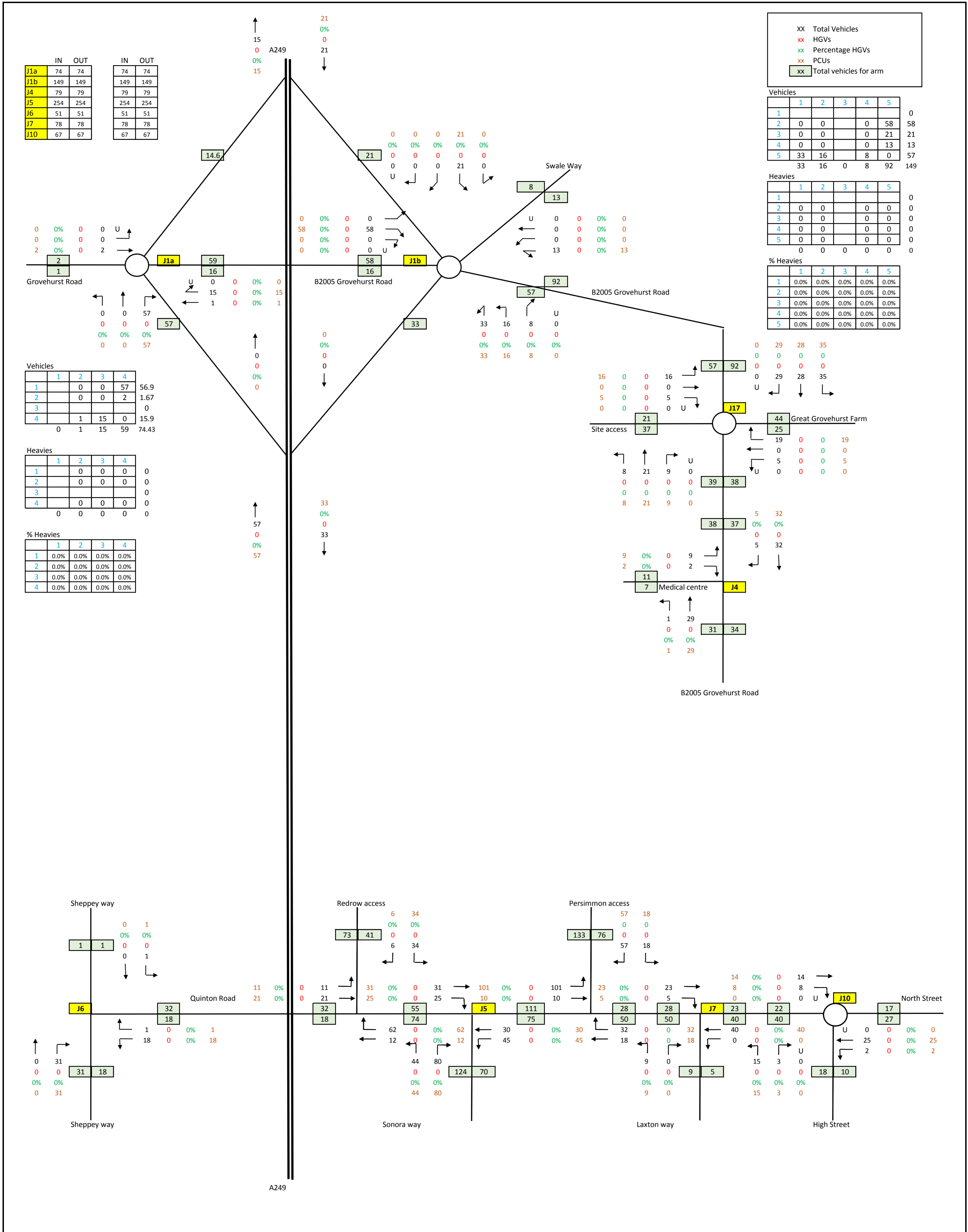
Total development flows - 2023 PM peak hour Sheet 1 of 2 Figure 8.2
