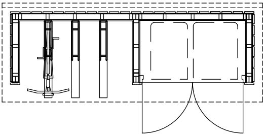
PROPOSED PLAN
