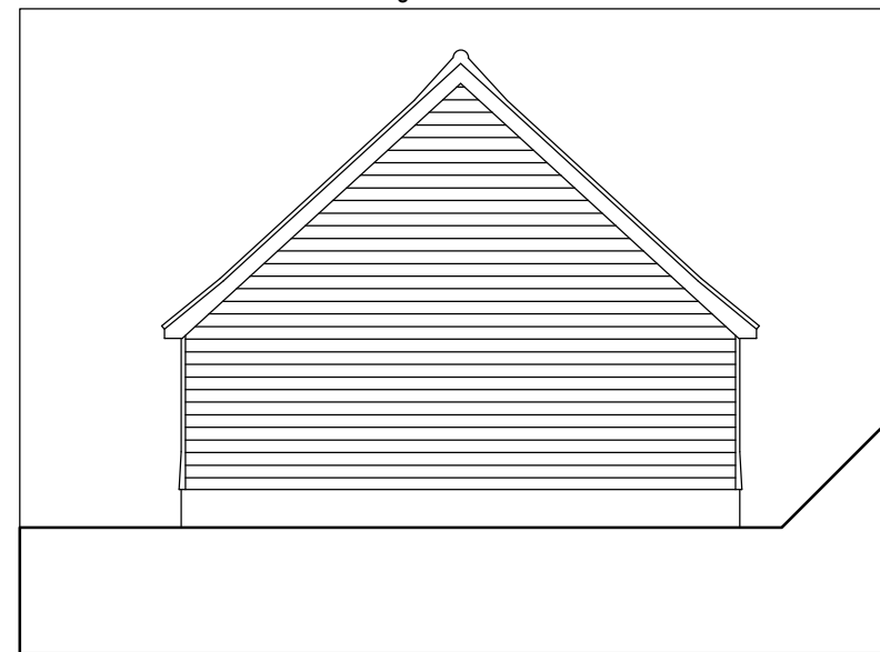
Unit 3 Garage Side Elevation 1:100
