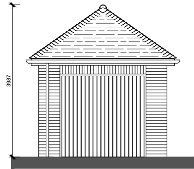
Garage Front Elevation (1:100 @A3)
