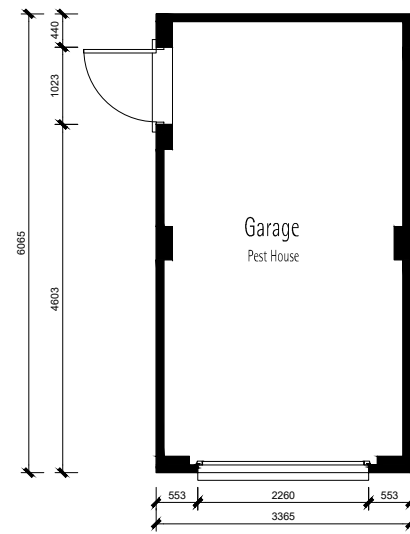
Garage Floor Plan (1:100 @ A3)
