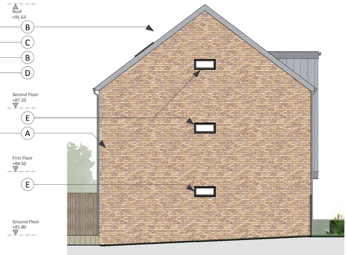
Block B - North Elevation
