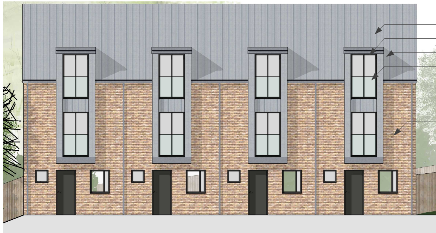
Block B - West Elevation
