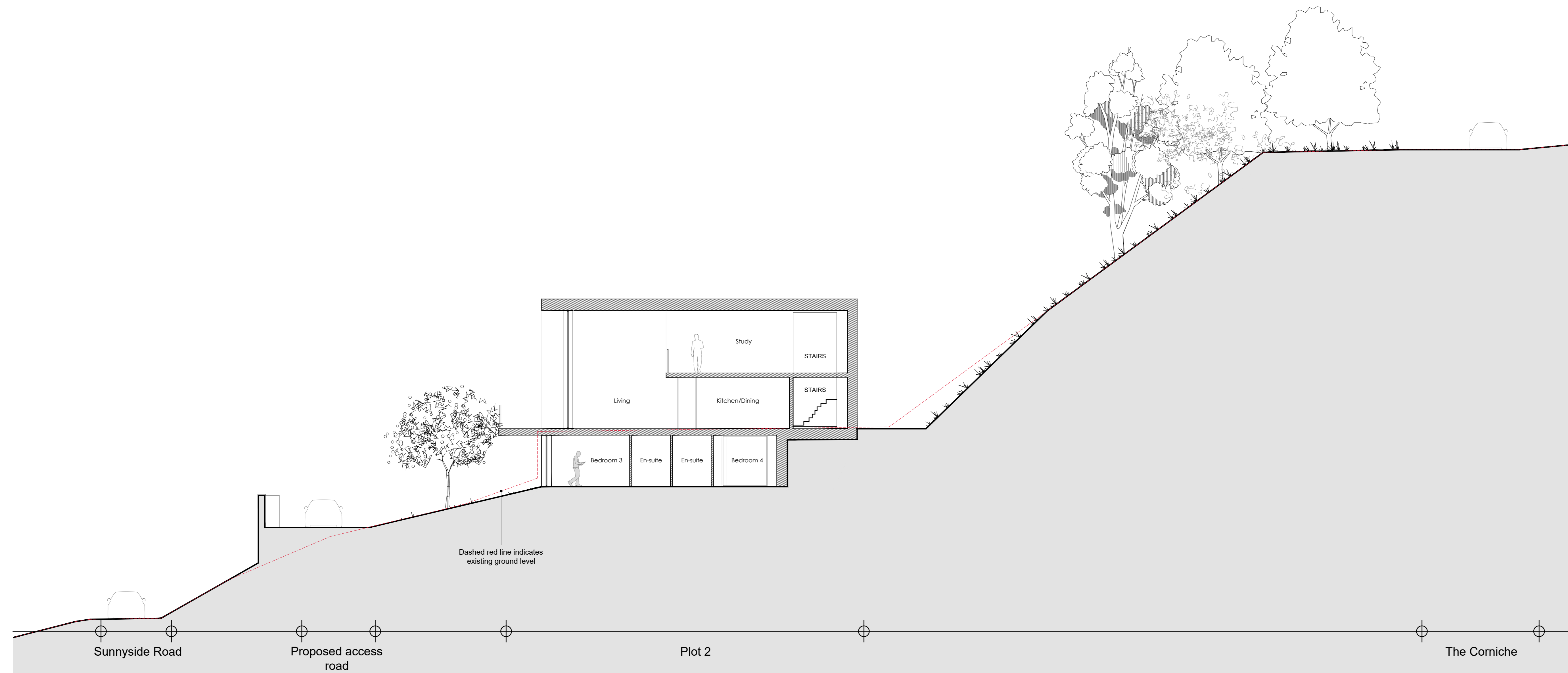
PLOT 2 SECTION @ 1:100 @A0
