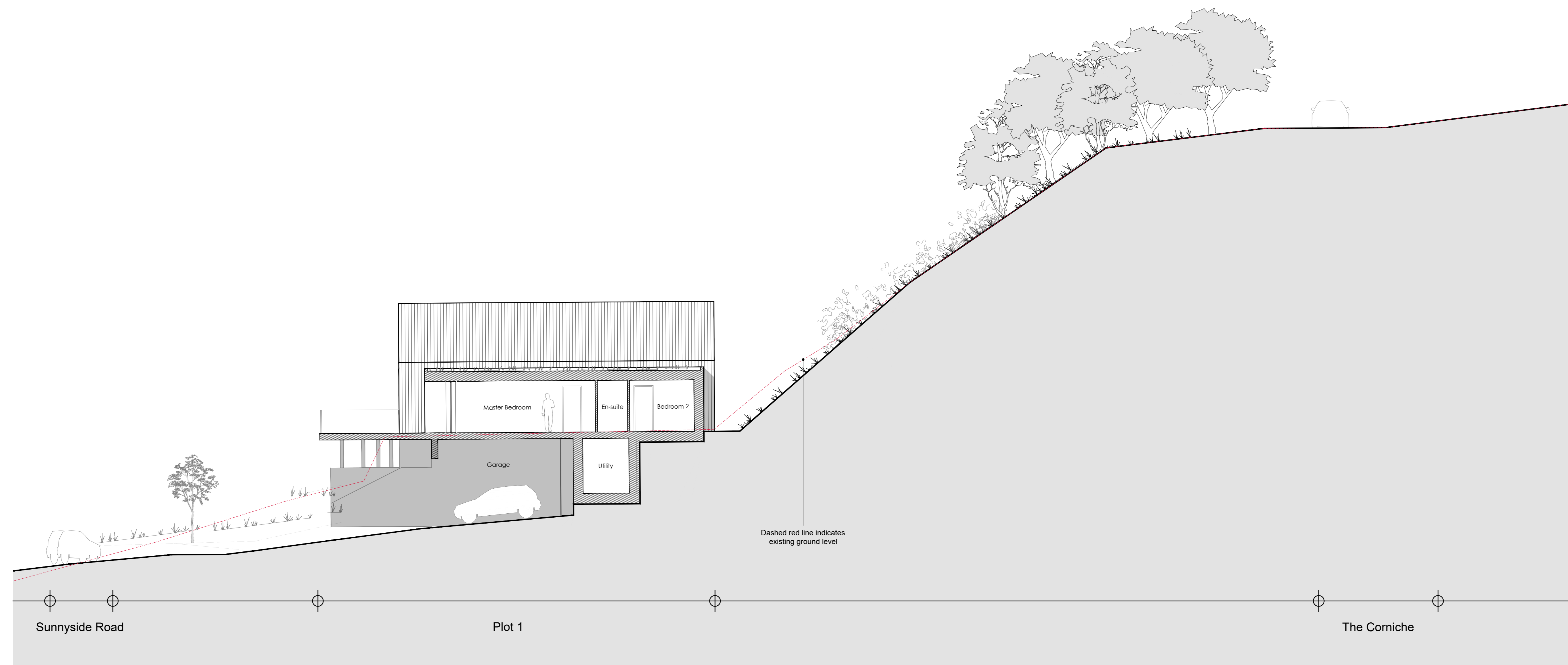
PLOT 1 SECTION @ 1:100 @A0
