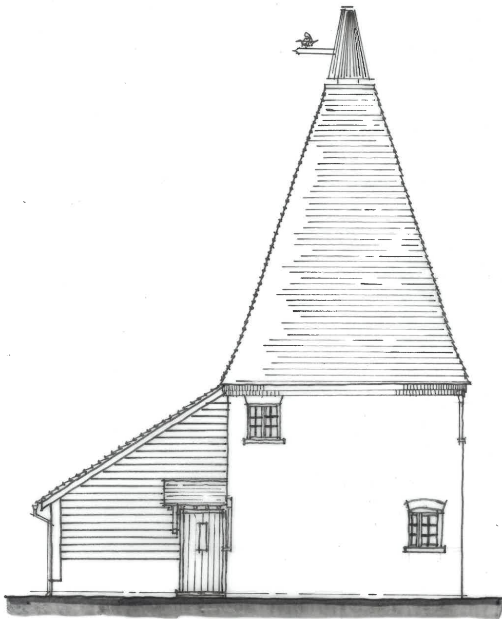
East Elevation
