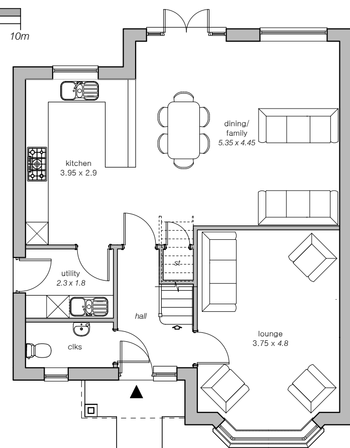
Ground Floor Plan 140sqm 4 bed 7p
