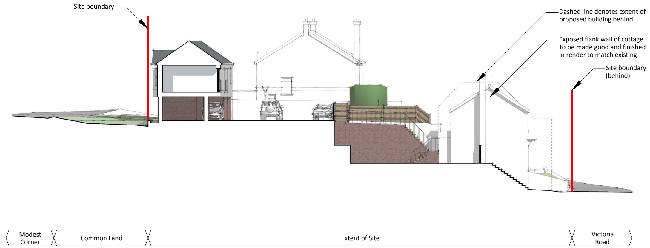
West Elevation of Laurel Cottage
