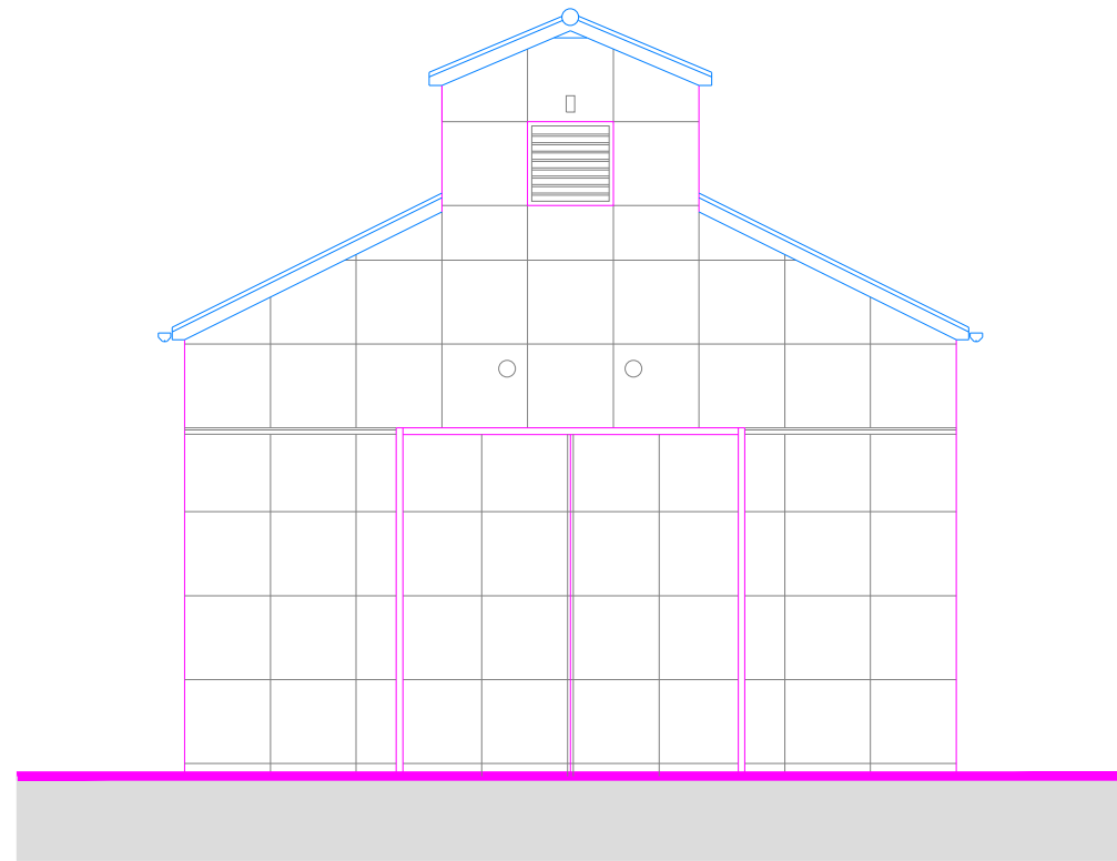
Existing South Elevation 1:100 @ A3
