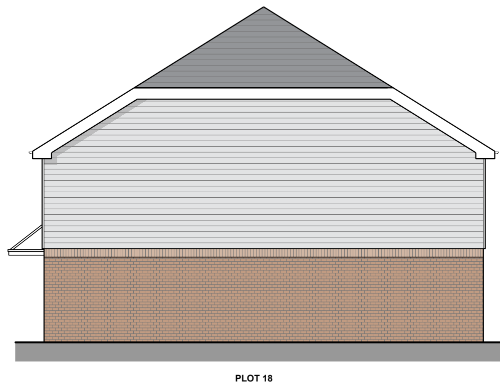
House Type 01 Elevation D
