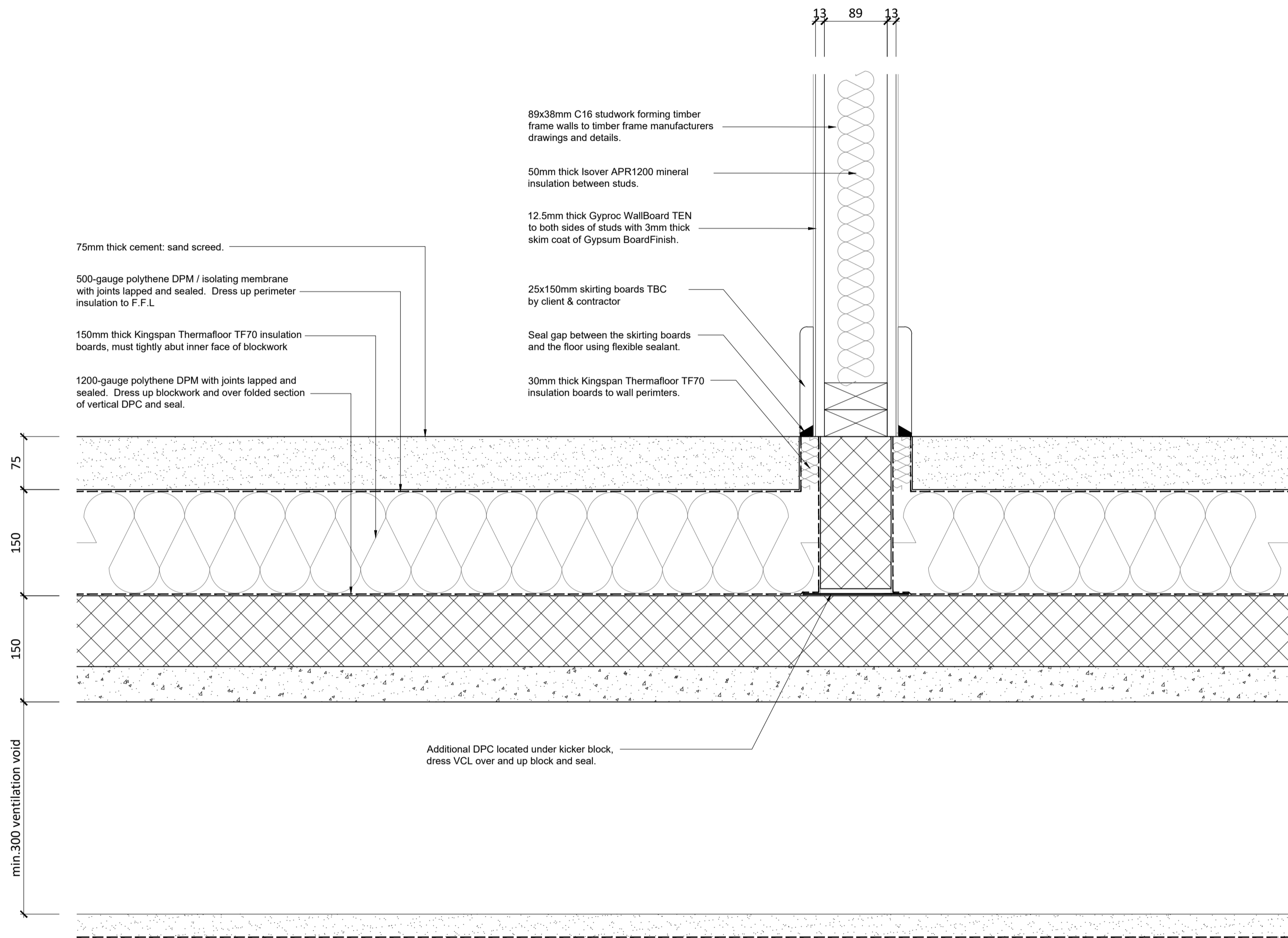
Detail 5 - Ground Floor / Internal Partition Detail 1:5
