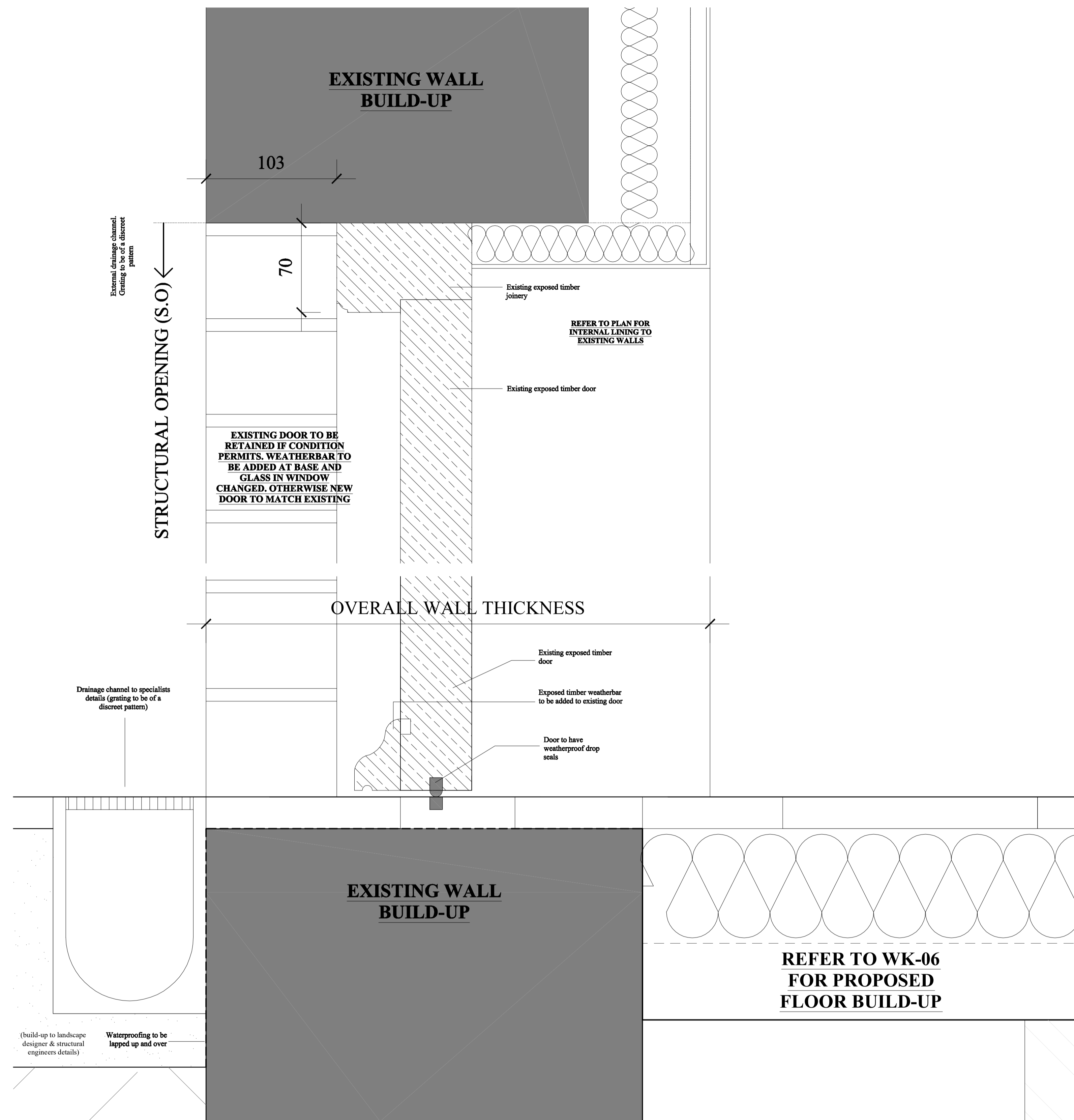
GF-D-01 SECTION DETAIL
