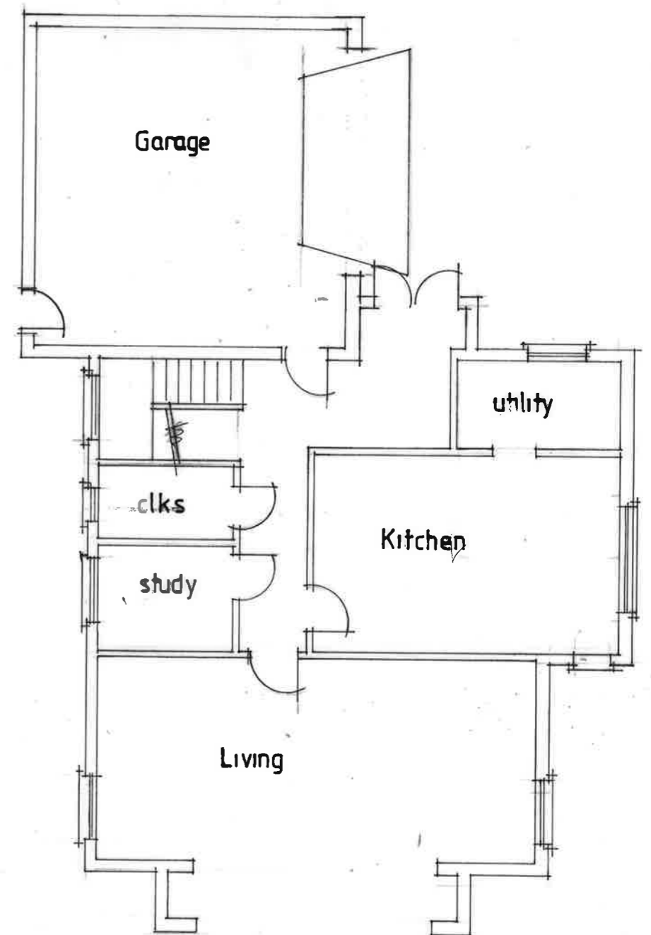
Ground Floor
