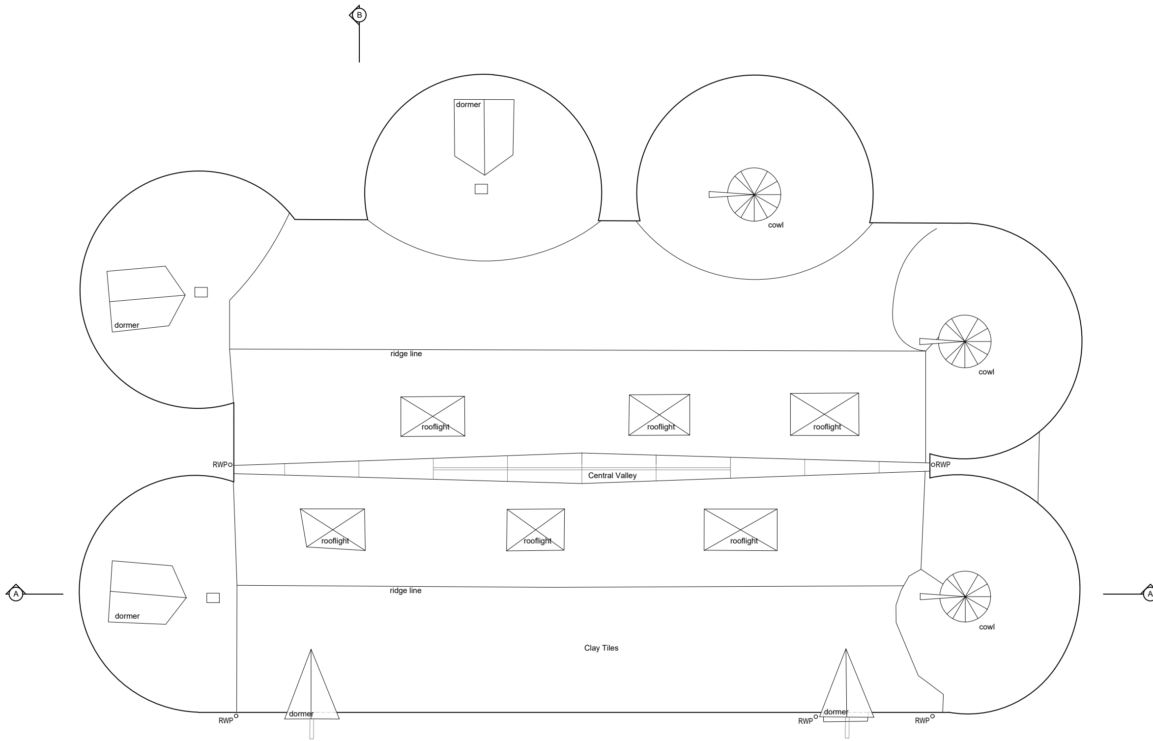
Roof Plan
