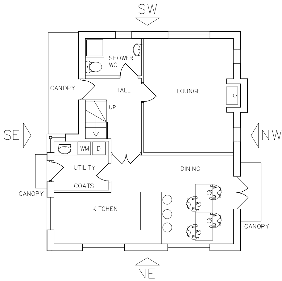
GROUND FLOOR (60 SQ M)
