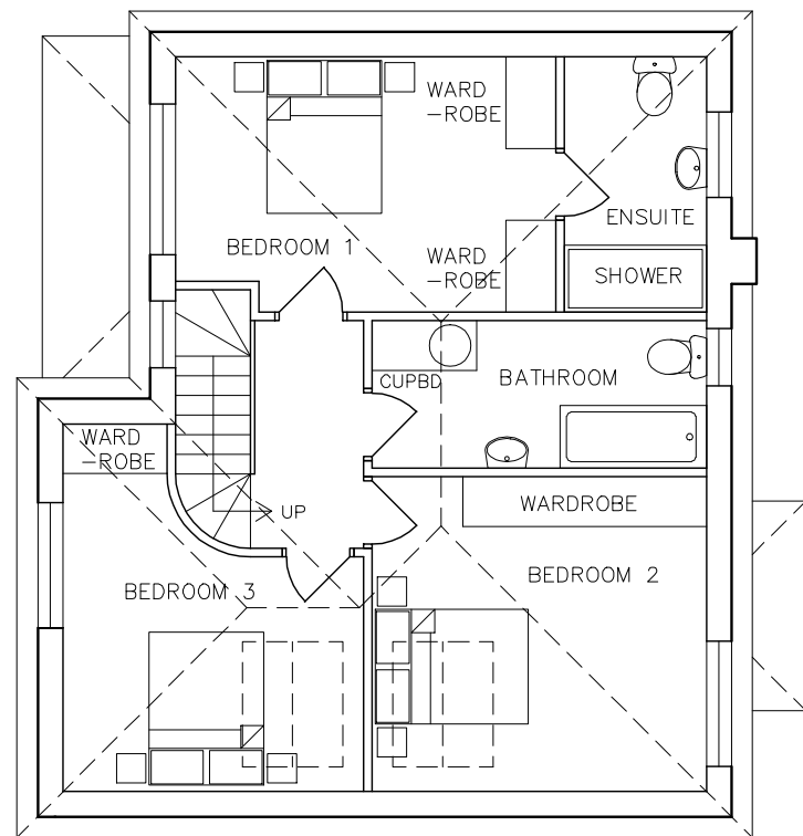
1ST FLOOR (60 SQ M)
