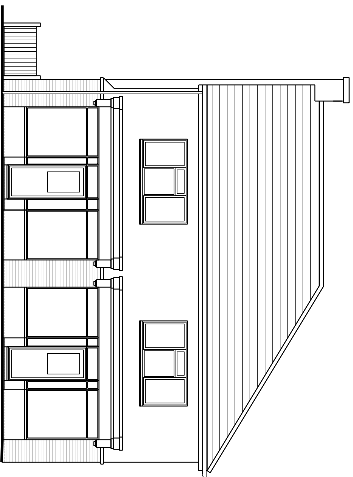
FRONT ELEVATION - SOUTH EAST
