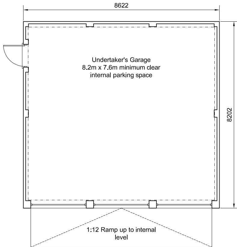
Garage Plan
