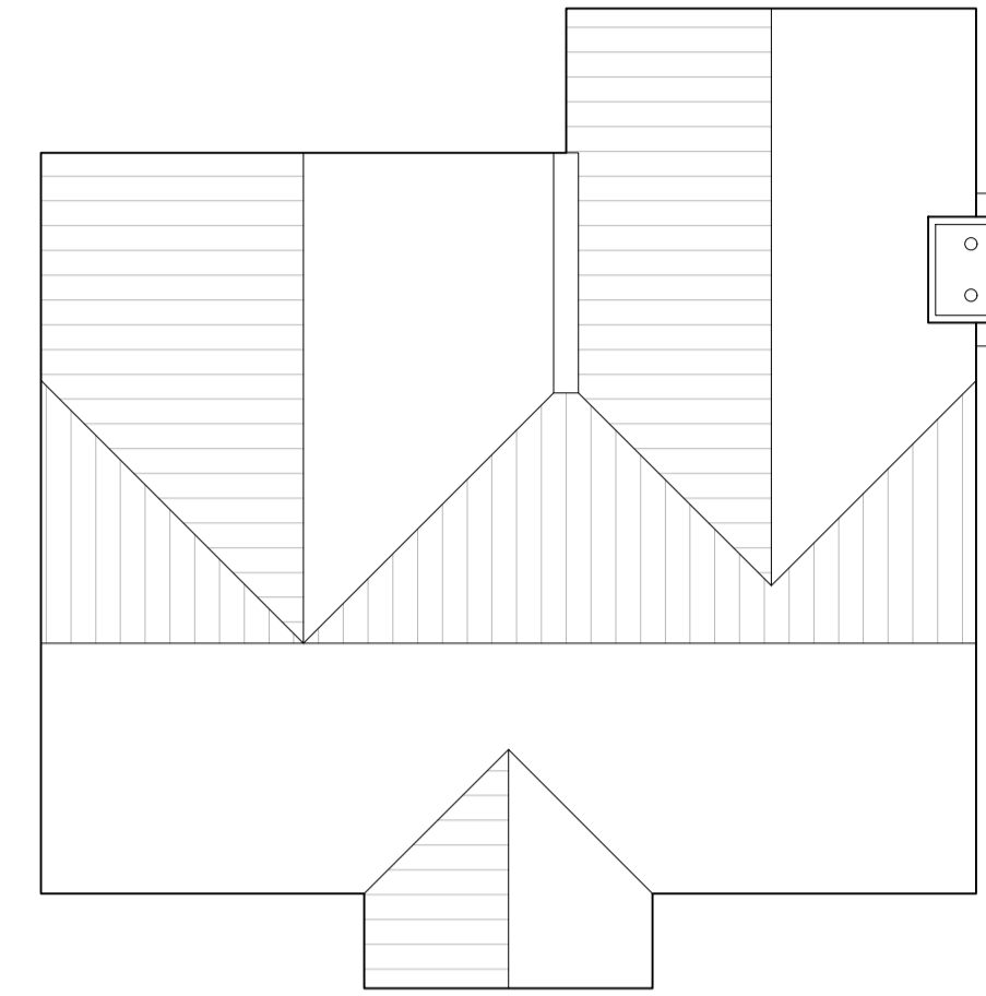
Roof Plan
