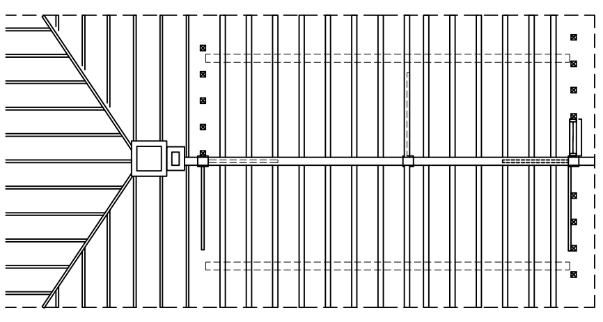
PLAN AT ROOF TRUSSES
